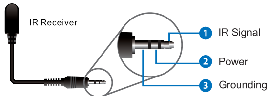
IR RECEIVER
