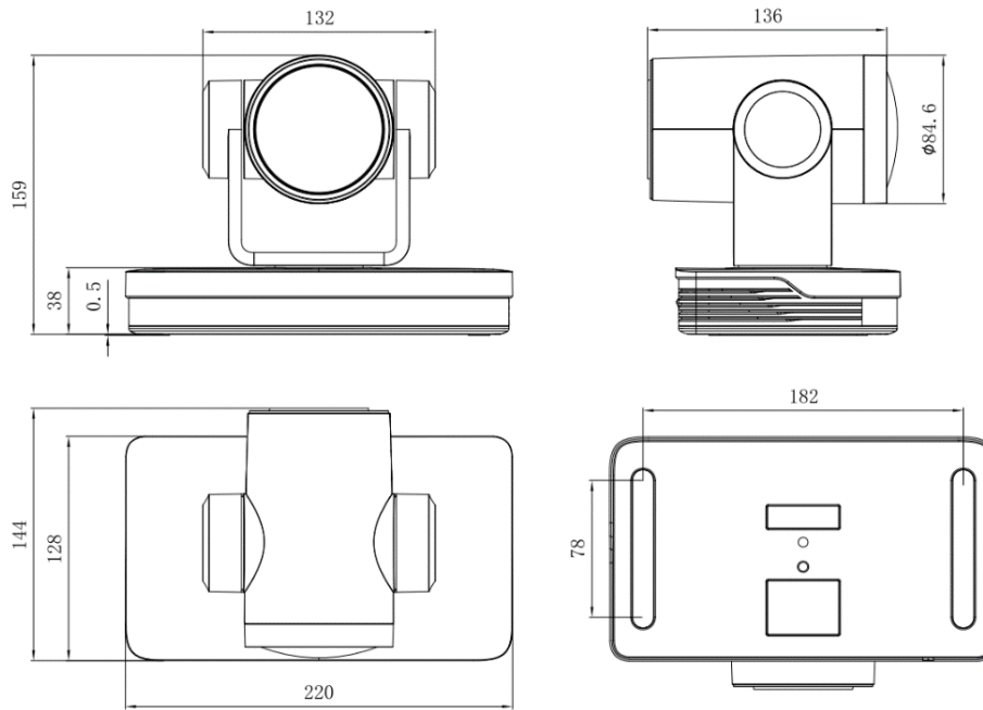
Figure1-4 Product Dimension
